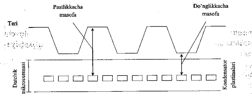
6.6-rasm. Sensor ishlashining prinsipi.
