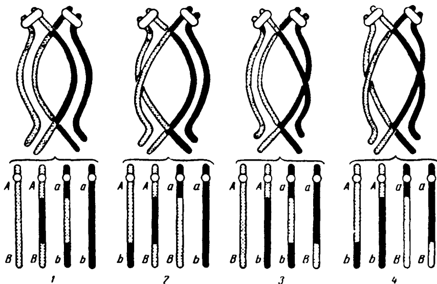
49-rasm. Xromosoma xromatidali o'rtasidagi qo'sh almashinish:
