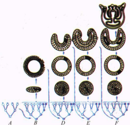
105-rasm. Ko'p hujayrali organizmlar ontogenezining bosqichma-bosqich murakkablashib borish sxemasi:
