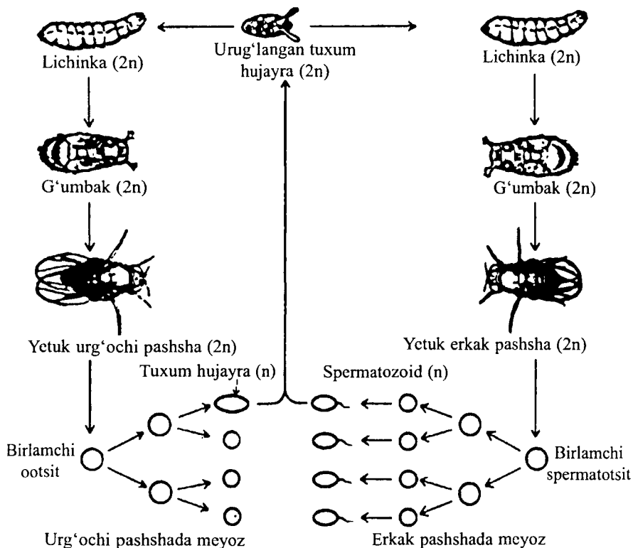
40-rasm. Drosophila pashshasida gametalarning hosil bo'lishi.
