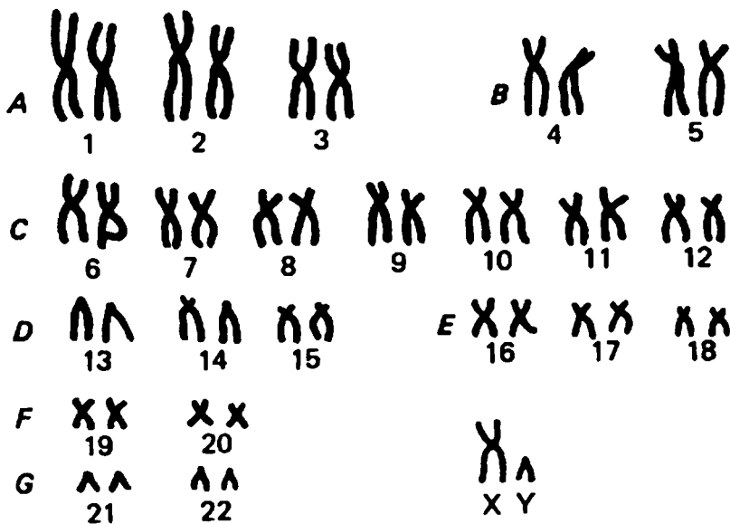
114-rasm. Erkak kishining xromosoma to'plami (A. A. Prokofyeva – Belgovskaya bo'yicha, 1969).
