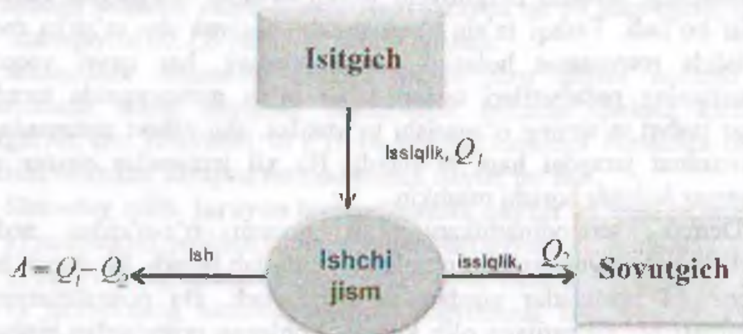
II.2-rasm. Issiqlikning ishga aylanishi
