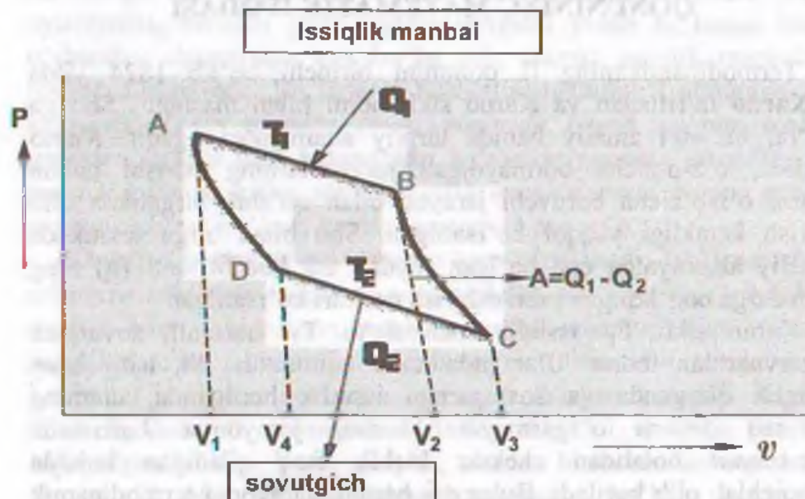
II.3 - rasm. Karno sikli
