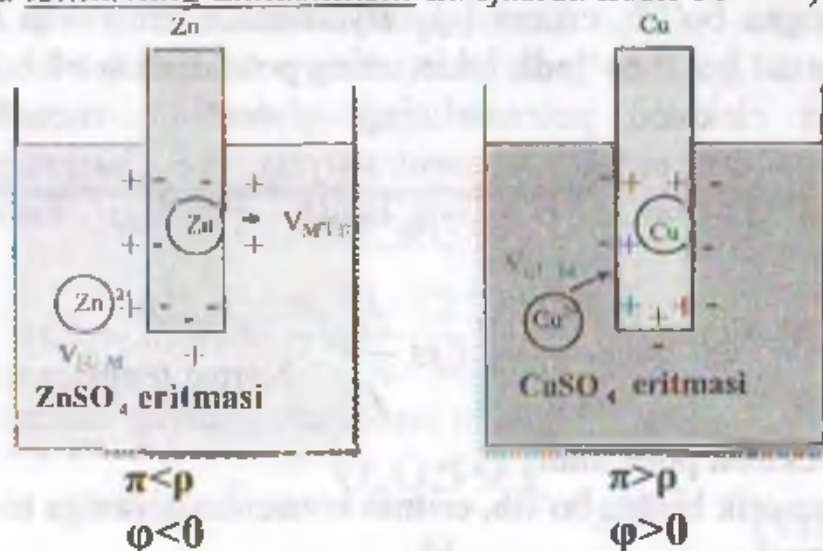
VIII.3-rasm. Elektrod potensiallarining hosil bo'lishi
