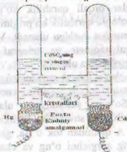
VIII.9 – rasm. Normal Veston elementining tuzilishi
