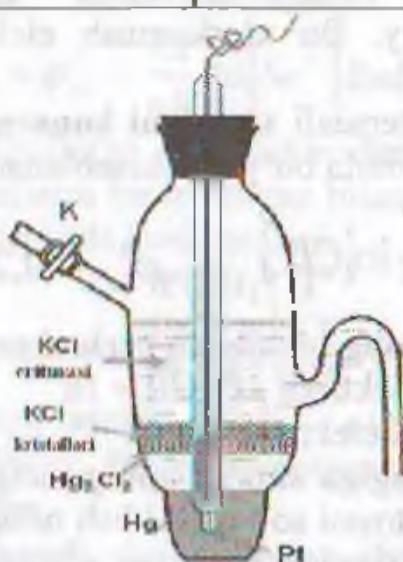
VIII.5 – rasm. Kalomel elektrodi
