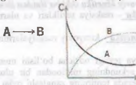
IX.1-rasm. Reagent (A) va reaksiya mahsuloti (B) konsentratsiyalarining vaqt birligida o'zgarishi
