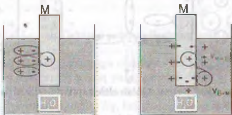
VIII.1-rasm. a). metall plastinkaning gidratlanishi;
