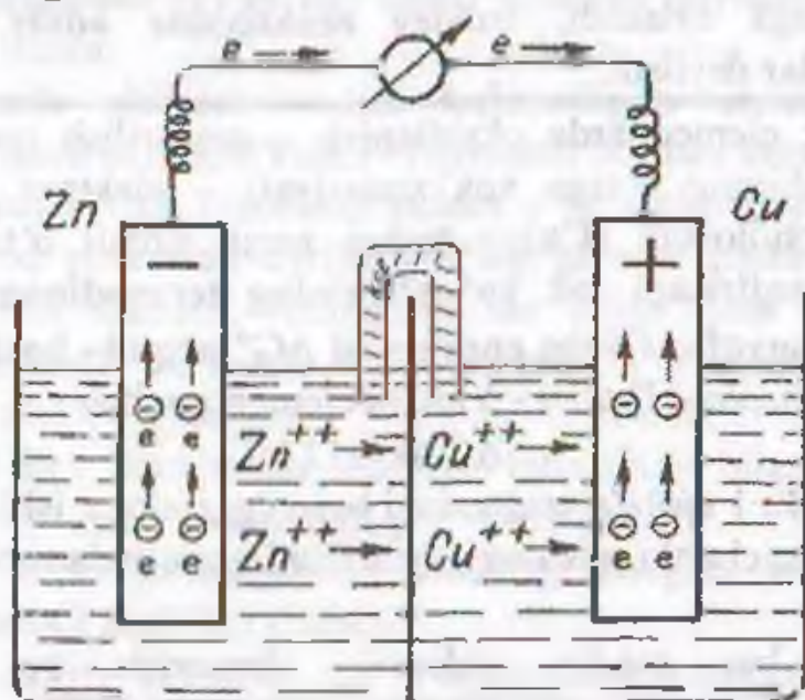
VIII.7 – rasm. Daniel – Yakobi galvanik elementi
