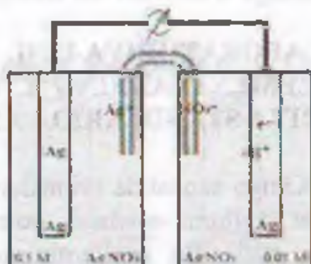
VIII.8 – rasm. Konsentratsion galvanik element
