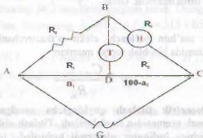
VII.5 – rasm. Kolraush ko'prigi sxemasi
