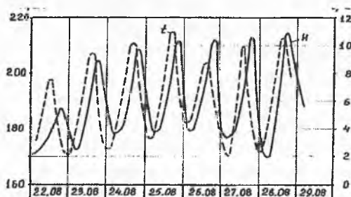
1.13.4-rasm. Zarafshon daryosining muzlikka yaqin qismida suv sathi (N) va harorati (t) ning tebranishi (L.K.Davidov ma'lumoti)
