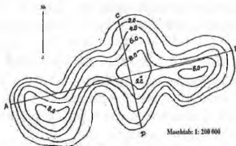
4.2-rasm. Kumushko'lning izobatlarida ifodalangan plani
