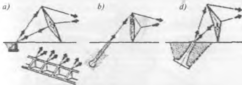
6.3- rasm. Tayanchning ankerli qurilmasi:
