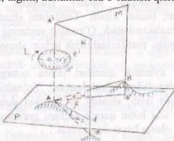
4.1-rasm. Gorizontol burchak o'lchash sxemasi
