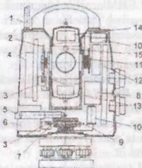
6.12-rasm. Elektron taxseometr tuzilishi sxemasi
