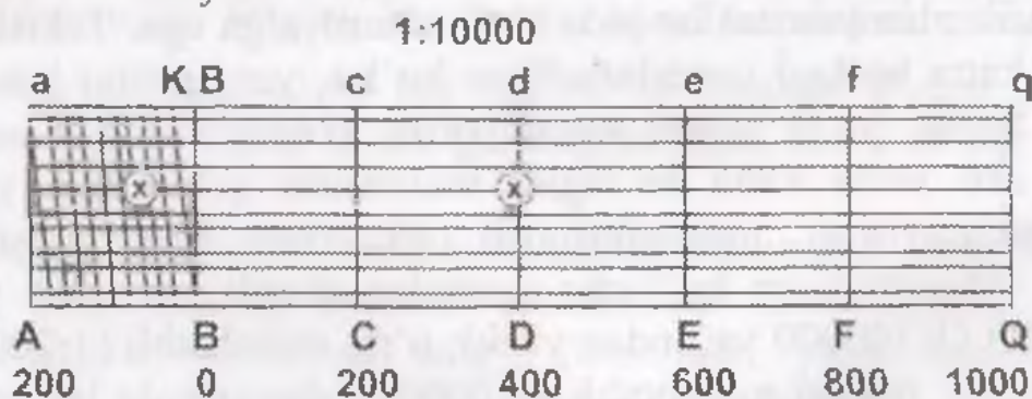
1.6-rasm. Ko'ndalang masshtab
