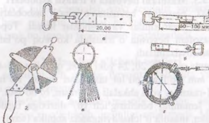
5.1-rasm. Masofa o'lchash qurollari
