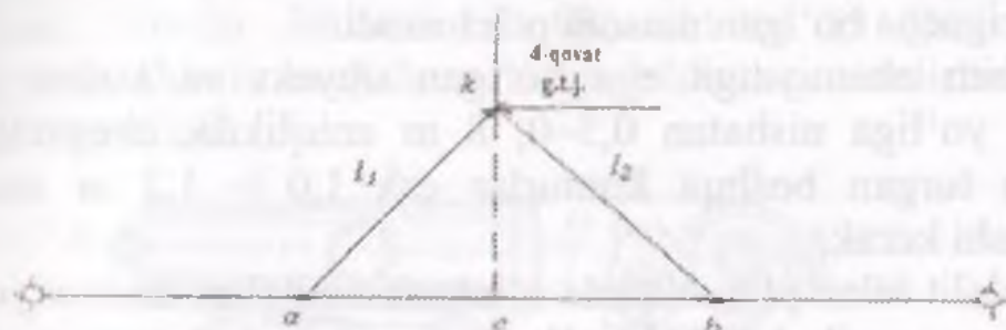
6.3-rasm. Chiziqli kestirma usuli
