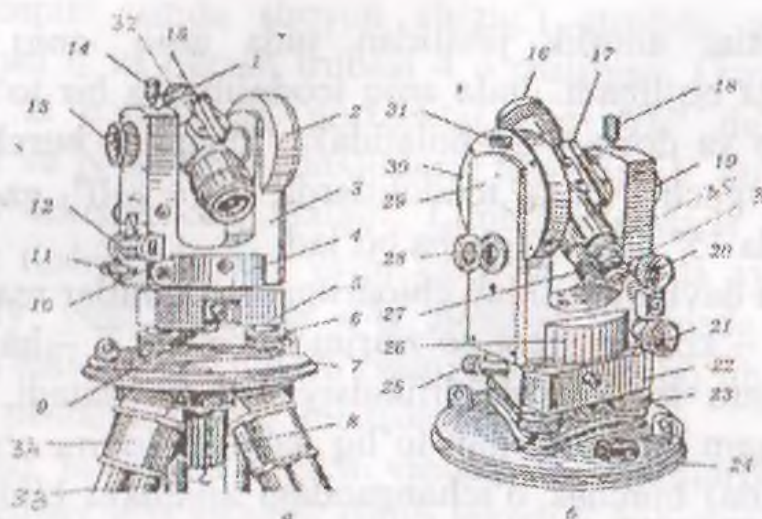
4.2-rasm. T30 teodolit tuzilishi
