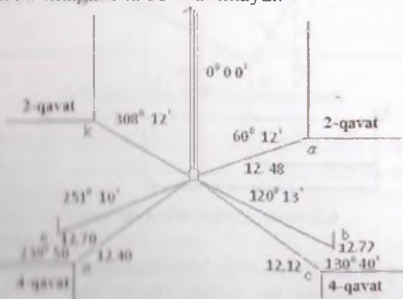
6.1-rasm. Qutbiy usulda planga olish
