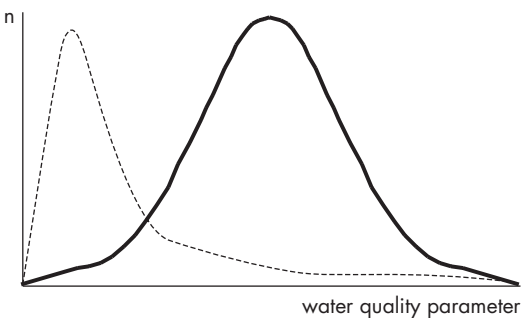
Figure 7.8 A log-normal distribution (broken line) compared to a normal distribution (solid line).
