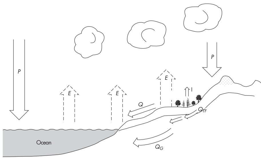
Figure 1.9 Processes in the hydrological cycle operating at the basin or catchment scale.
