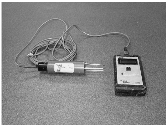
Figure 4.11 The Theta probe (manufactured by Delta-T devices). An example of a small, time domain reflectometry instrument used to measure soil moisture content in the field. The metal spikes are pushed into the soil and the moisture level surrounding them is measured.
