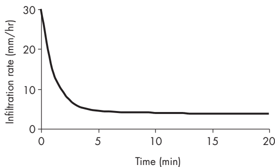
Figure 4.3 Typical infiltration curve.
