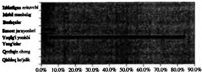
16-rasm. \text{SO}_2 ajrab chiqishining manbalari.
