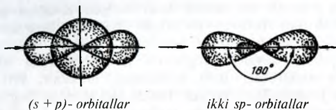
2.2- rasm. Valent orbitallarning sp - gibridlanishi.
