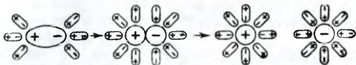
4.2- rasm. Eritmada qutbli molekullarning dissotsilanishi.
