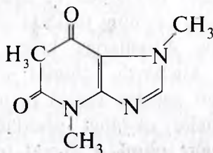
kofein (1,3,7-trimetilksantin)
