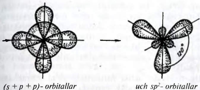
2.4- rasm. Valent orbitallarining sp^2 - gibrizlanishi.
