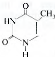
timin
