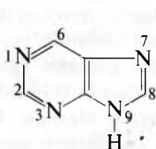
purin
