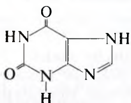
ksantin (2,6-dioksipurin)
