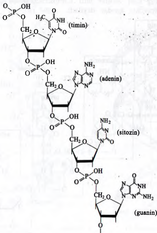
16.4-rasm. DNK molekulasi fragmentining tuzilishi.
